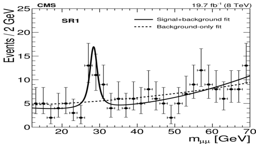
Fig.6. Peak of energy at 28GeV
