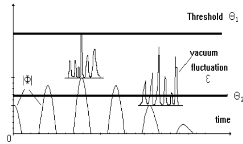
Fig.4. Quantum measurements.
