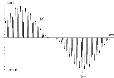
Fig. 2. Behavior of wave packet in linear dispersion medium (i.e., rather like a series of stroboscopic photographs).
