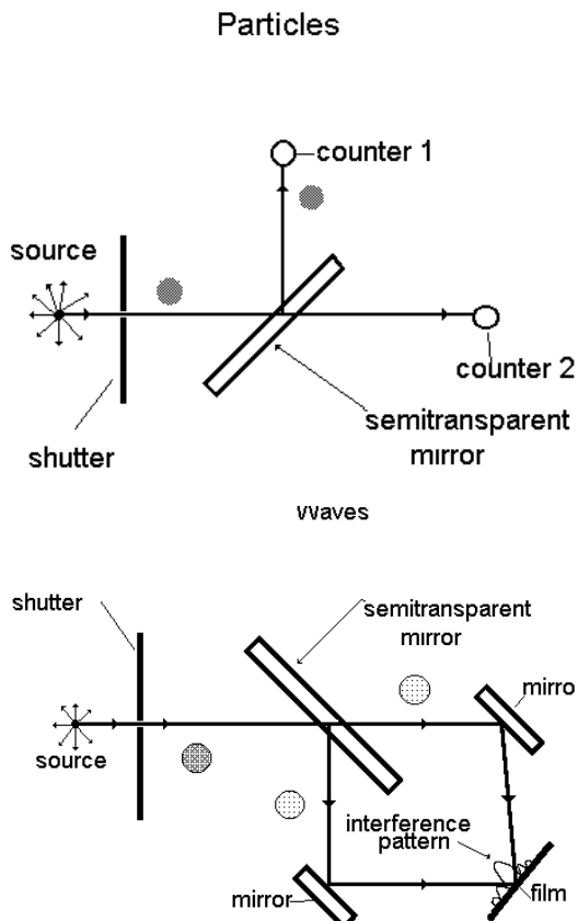
Fig.1. Experiments with individual photons on semitransparent mirror.
