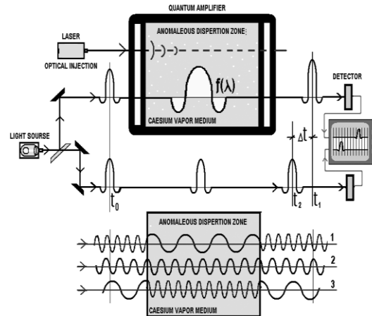
Fig. 5. Experiments of L.Wang - superluminal light propagation.
