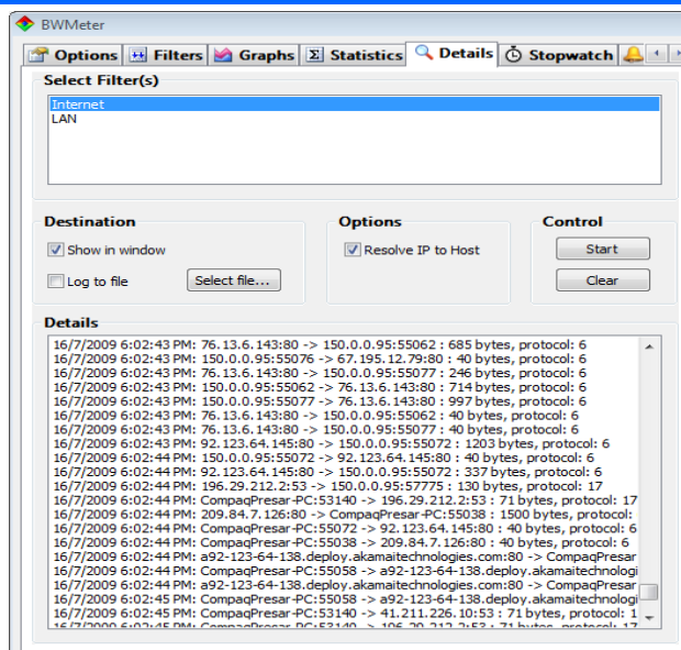
Fig. 3. Details menu of Bandwidth Meter
