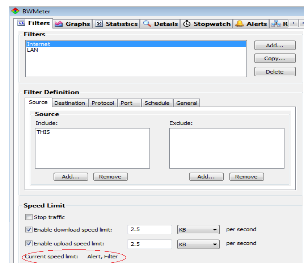
Fig. 4. Setting speed limit in Bandwidth Meter
