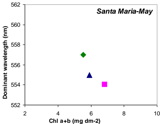
Fig 5. Decrease of the dominant wavelength with increasing of chlorophyll content of different type of leaves, from shade leaf to sun leaf, of the Santa Maria variety on May.
