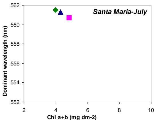
Fig. 6. Decrease of the dominant wavelength with increasing of chlorophyll content of different type of leaves, from shade leaf to sun leaf, of the Santa Maria variety on July.
