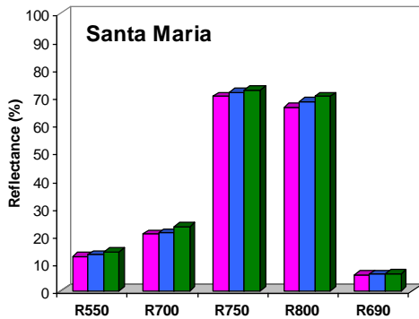
Fig. 2. Values reflectance of the sun (south part), blue-shade (north part) and shade/half shade leaves of Santa Maria pear variety on May(upper side).
