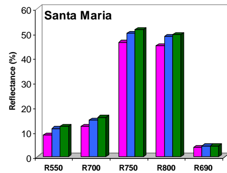
Fig. 4. Values reflectance of the sun (south part), blue-shade (north part) and shade/half shade leaves of Santa Maria pear variety on July (upper side). Mean of 6 reflectance spectra per leaf-type.
