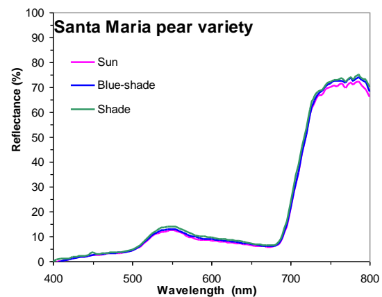
Fig. 1. Reflectance spectra of the sun (south part), blue-shade (north part) and shade/half shade leaves of Santa Maria pear variety on May (upper side). Mean of 6 reflectance spectra per leaf-type.
