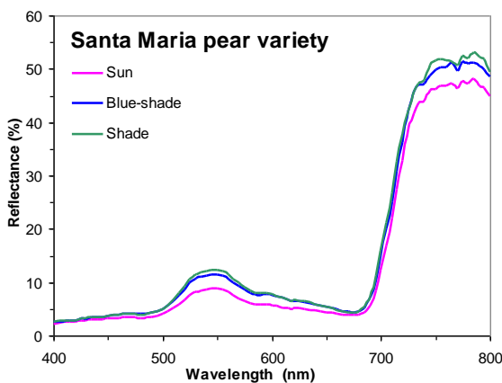
Fig. 3. Reflectance spectra of the sun (south part), blue-shade (north part) and shade/half shade leaves of Santa Maria pear variety on July (upper side). Mean of 6 reflectance spectra per leaf-type.
