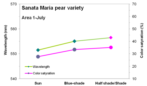
Fig. 7. (A), (B). Dependence dominant wavelength, color saturation for three positions; sun, blue shade and shade
